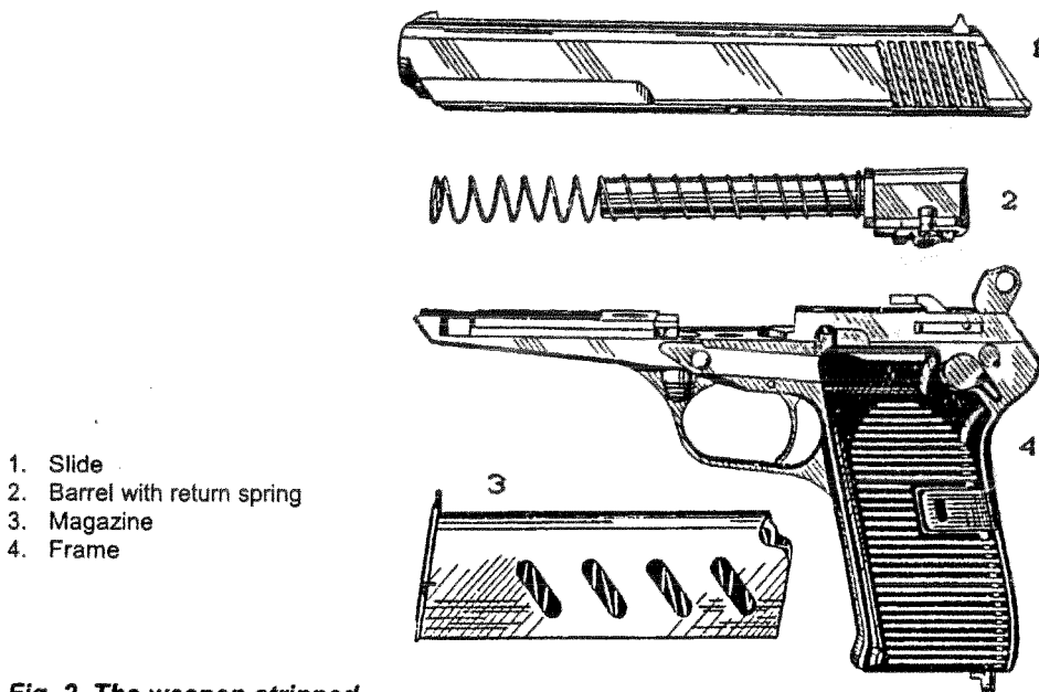
Fig. 2 The weapon stripped
