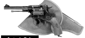
Russian Nagant M1895 Revolver, Cal. 7.62 Nagant
